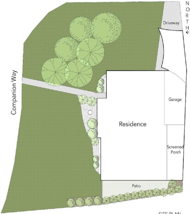
SITE PLAN
